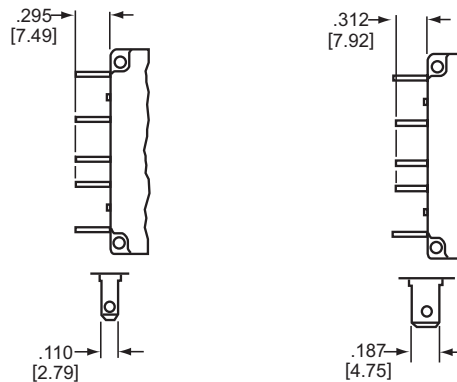
Auxiliary Switch
