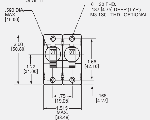
UPGH11
