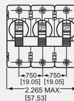
UPGH 111
