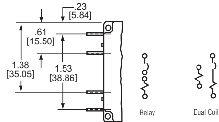
Relay and Dual Coil
