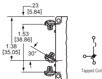
Tapped Coil
